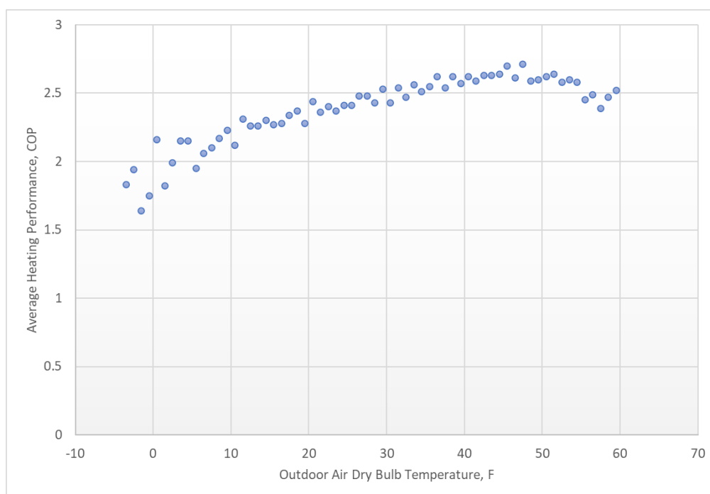
Figure 6. Overall Average Seasonal Heating Performance by Outdoor Air Temperature
