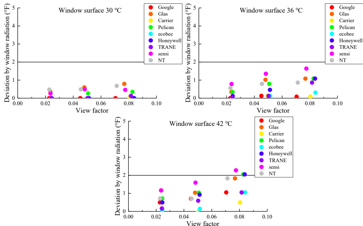
Figure 8. Thermostat deviations in the thermal asymmetry testing, for exposure to a heat panel simulating a window surface: at 30C, 36C and 42C.
