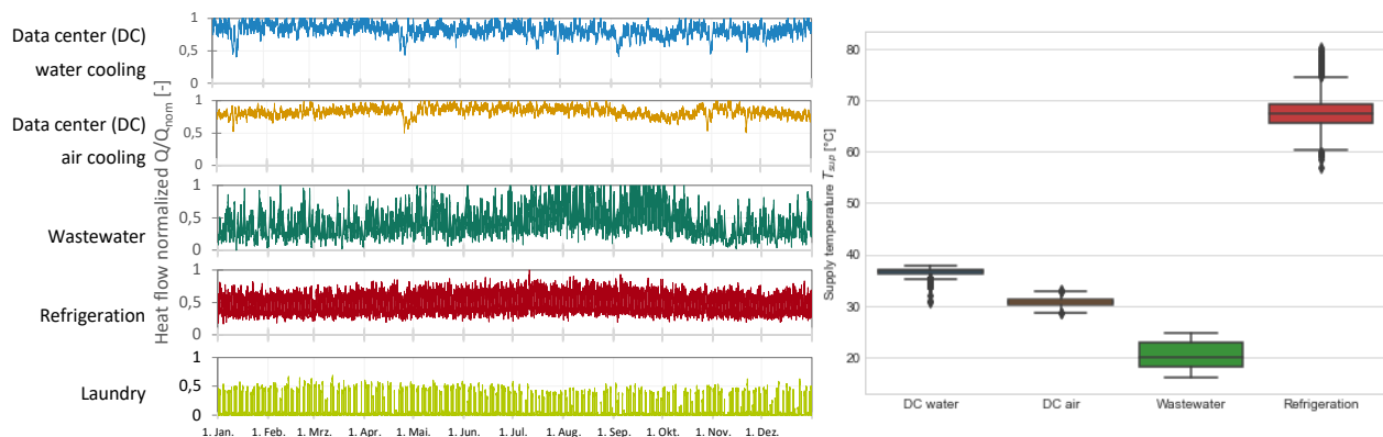
Figure 2: Heat flow and temperature profiles of five different types of waste heat sources.
