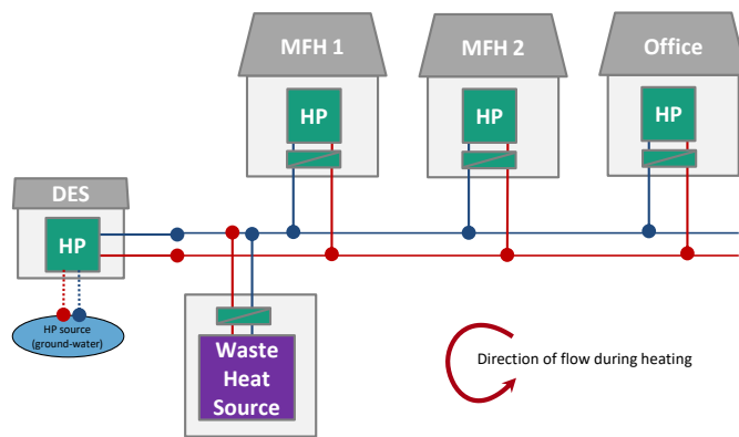
Figure 3: Hydraulic integration of a waste heat source in the 5GDHC network by an increase of return temperatures to the district energy system (DES).
