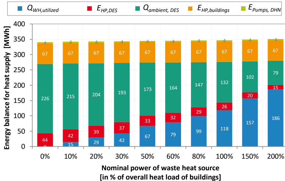
Figure 5: Energy balance of the 5DHC network with varying nominal power of the waste heat source.
