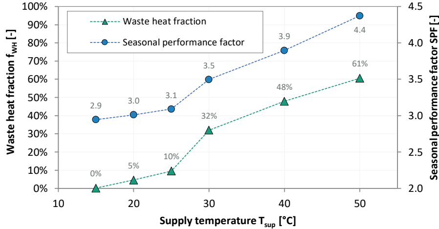
Figure 7: Waste heat fraction and seasonal performance factor with varying quality of waste heat in terms of supply temperature T_{sup} for an open waste heat process.
