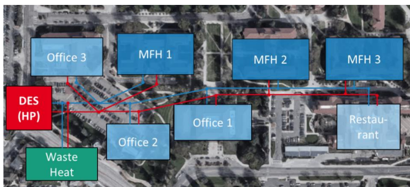
Figure 1: Model district consisting of three residential multi-family houses (MFH), three office buildings, a restaurant, and a central ground-source heat pump (HP) in the district energy system (DES). Waste heat is integrated in the cold return pipe to the central heat pump. Background image: © CNES / Airbus, Maxas Technologies, I.S. Geological Survey, USDA/FPAC/GEO, Google
