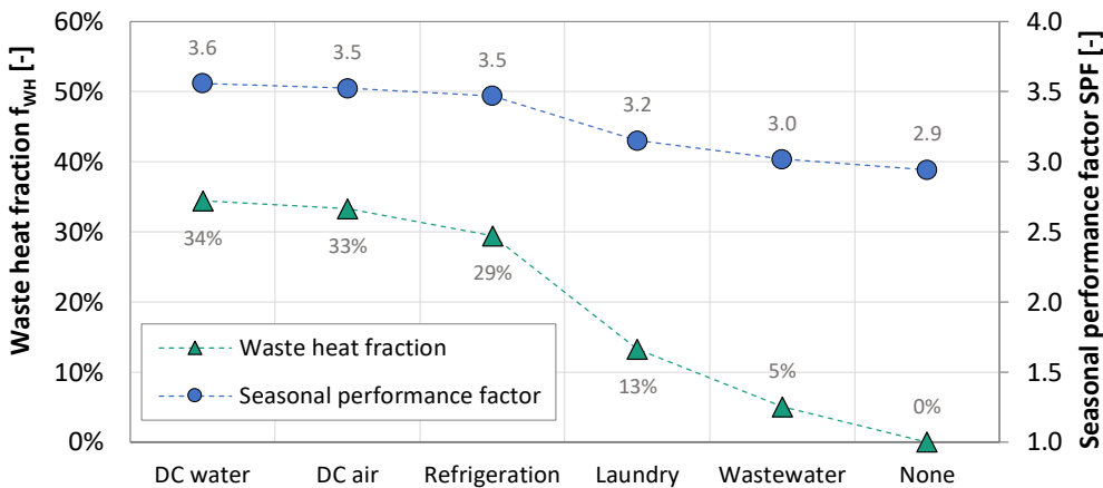
Figure 8: Waste heat fraction and seasonal performance factor for varying waste heat sources with equal annually available waste heat
