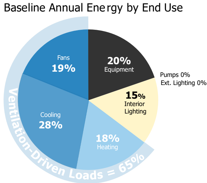
Figure 1 Energy use by end-use type in a typical laboratory building. Values were calculated from the OpenStudio energy model developed for the NREL Research and Innovation Laboratory (Group 14 Engineering, PCB 2021). (Image Credit: Amanda Kirkeby, NREL)
