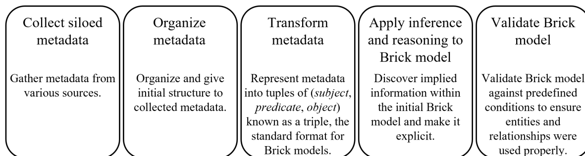
Figure 3: The five-step workflow process to develop a Brick model for a building.
