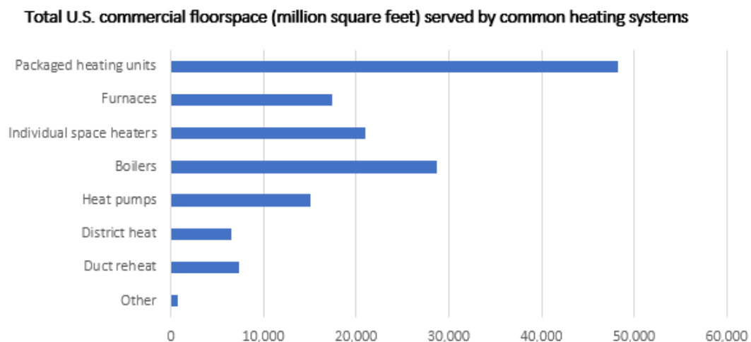
Figure 2: Common commercial building heating systems (US EIA 2018).
