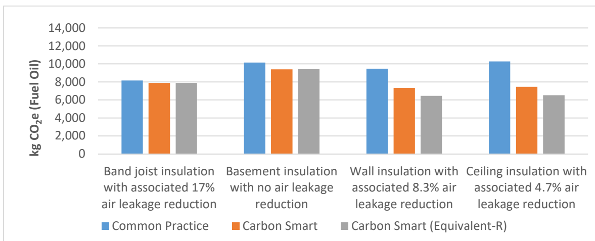
Figure 6. First-year operational and embodied CO 2 e emissions, in kilograms, by measure.
