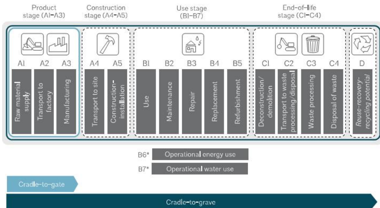
Figure 1. Life cycle stages for building products (Lewis et al. 2021).
