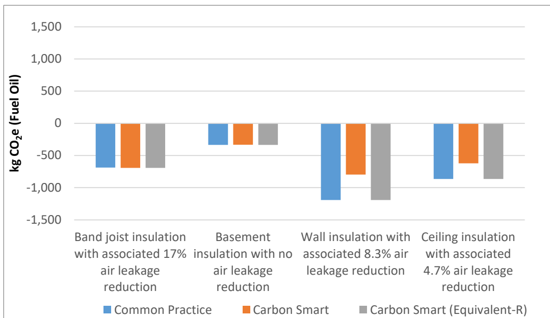
Figure 4. First-year operational savings of CO 2 e, in kilograms, by measure, compared to the Baseline.
