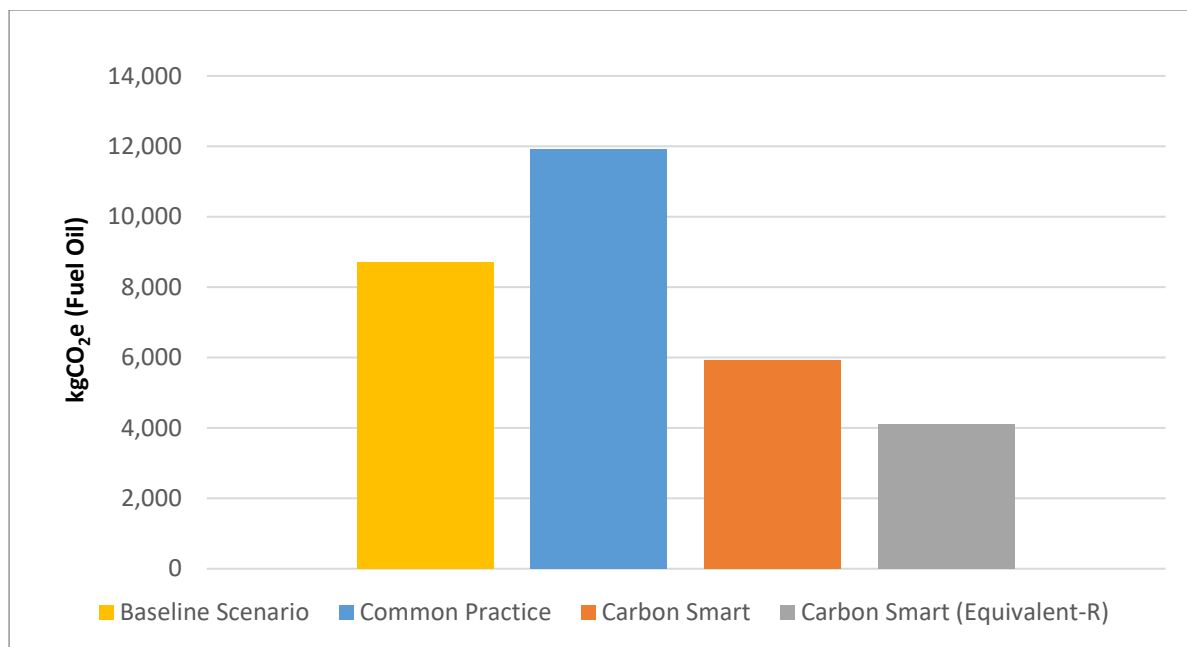
Figure 5. First-year operational and embodied CO 2 e emissions, in kilograms, for a weatherized house, all measures.
