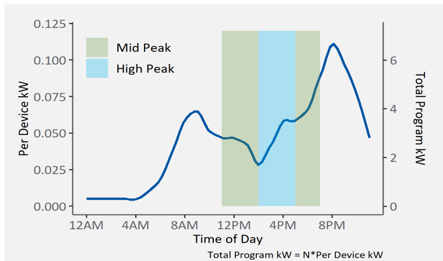
Figure 10. Dryer Average Summer Demand Profile. Source: Cadmus.
