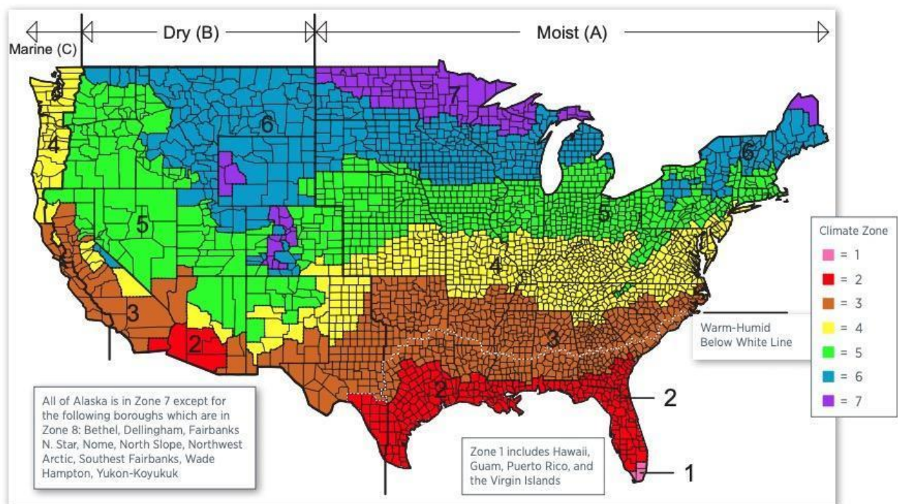
Figure 1. International Energy Conservation Code (IECC) climate regions of the United States.
