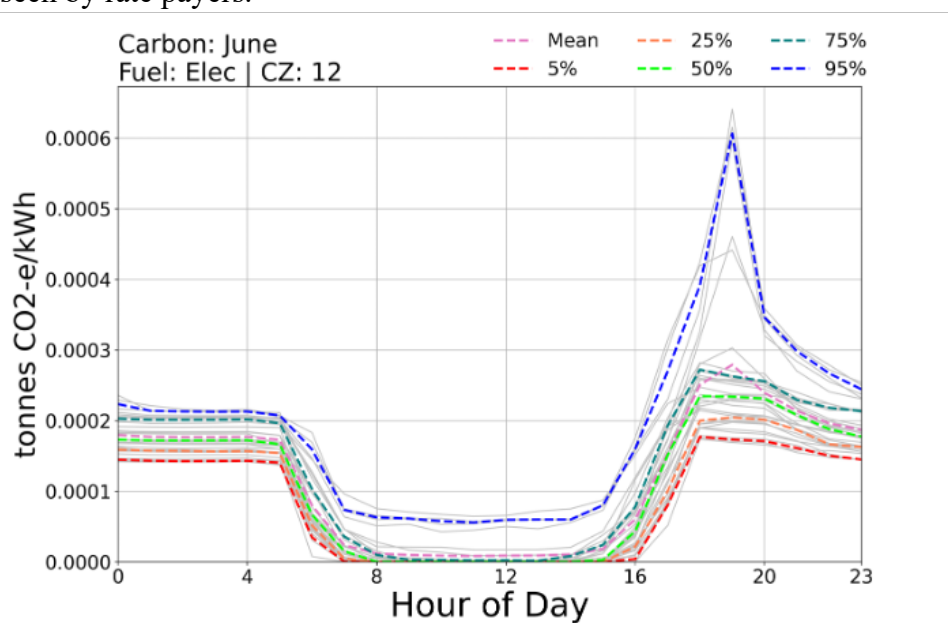
Figure 1. CO 2 emissions factors for June in California Climate Zone 12 (Northern California Central Valley). Each gray line represents a single day, and the colored lines represent the mean and percentile values across all days.
