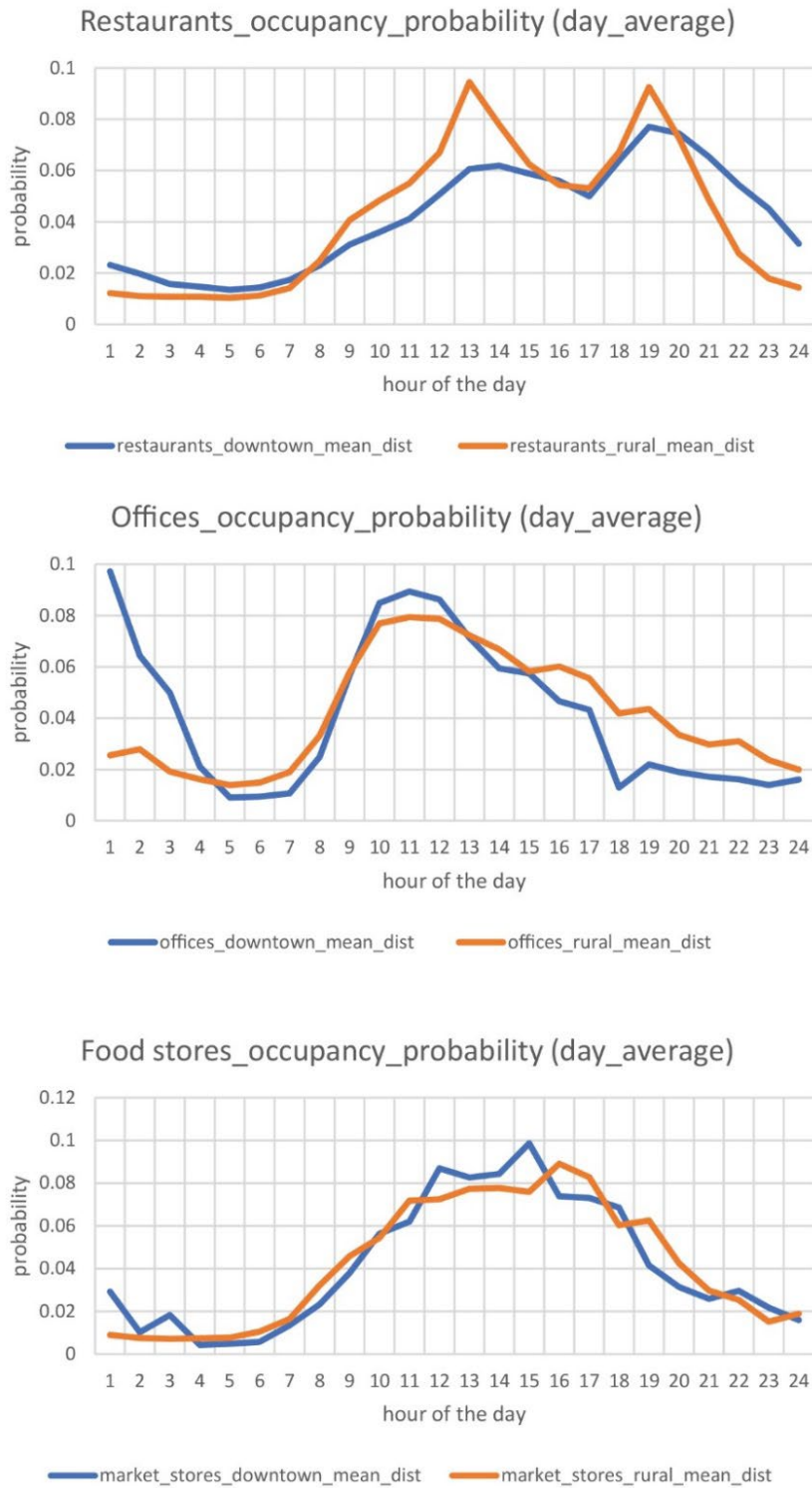
Figure 8 - Occupancy probability distribution comparison between the downtown and rural areas
