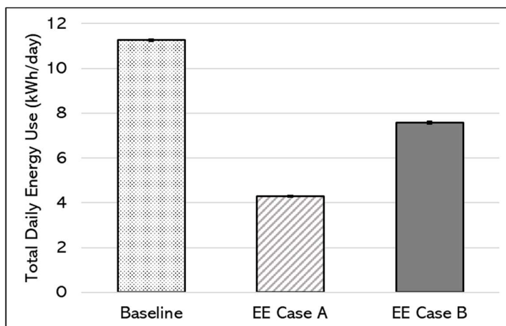
Figure 4. Total mean daily energy consumed by each of the three refrigerator case technologies. Error bars indicate standard deviation across individual 24-h experiments (negligible).
