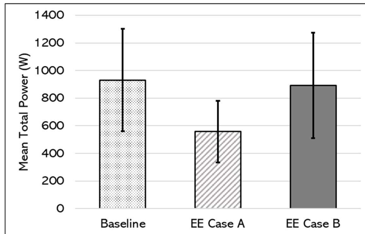
Figure 6. Mean power consumed by each of the three refrigerator cases' components during compressor on-cycling. Error bars indicate standard deviation across total compressor on-cycle time.
