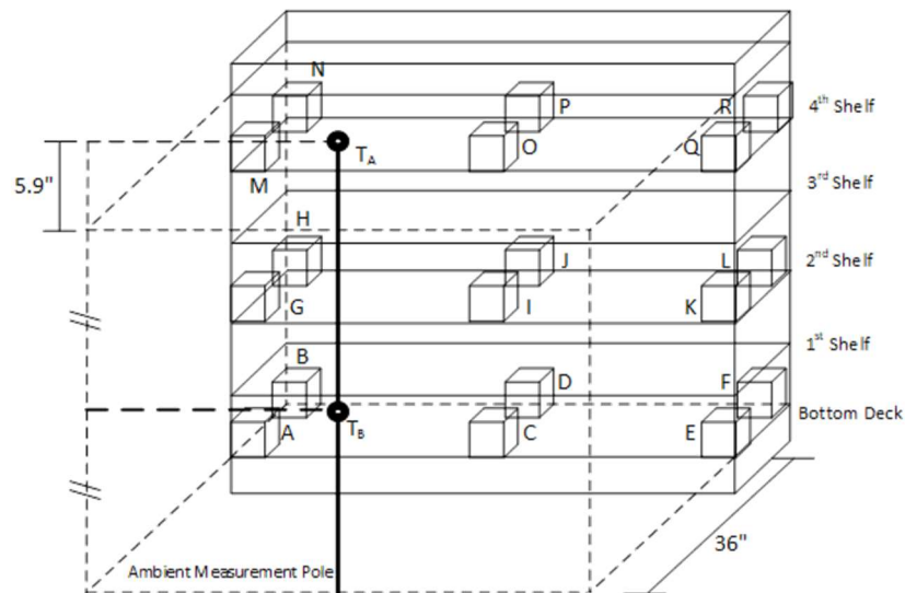
Figure 3. Schematic of product simulator temperature measurement locations (A–R), and ambient temperature locations ( T_A and T_B )
