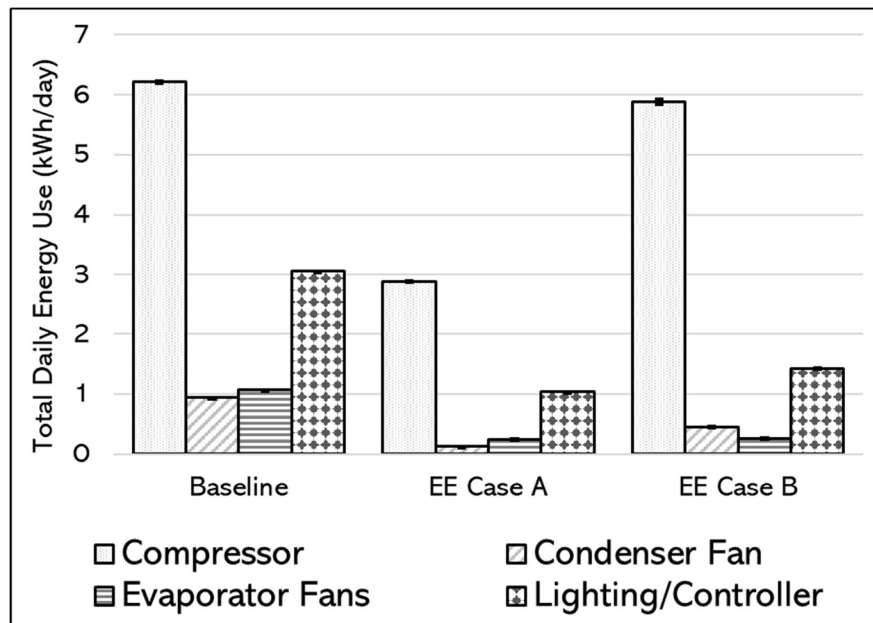
Figure 5. Mean daily energy consumed by each of the three refrigerator cases’ components. Error bars indicate standard deviation across individual 24-h experiments (negligible).
