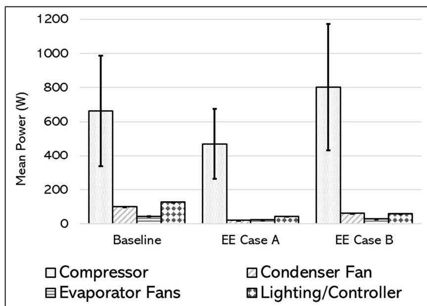
Figure 7. Mean power consumed by each of the three refrigerator cases' components during compressor on-cycling. Error bars indicate standard deviation across total compressor on-cycle time.
