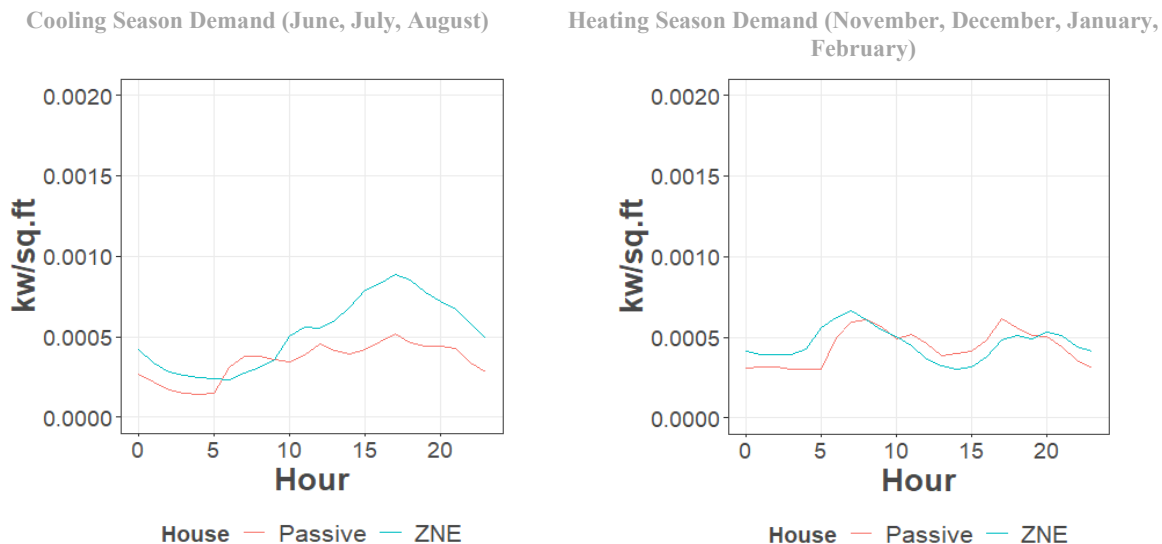
Figure 2. Passive House and ZNE Seasonal Load Comparisons
