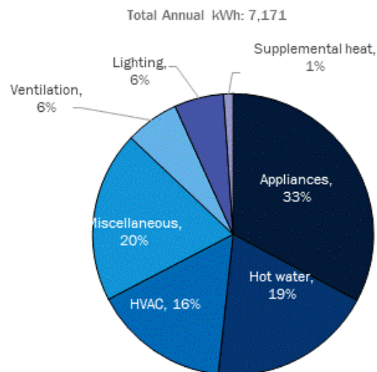
Figure 1. Passive House Energy Consumption. Based on the disaggregated load of two Passive Houses in California
