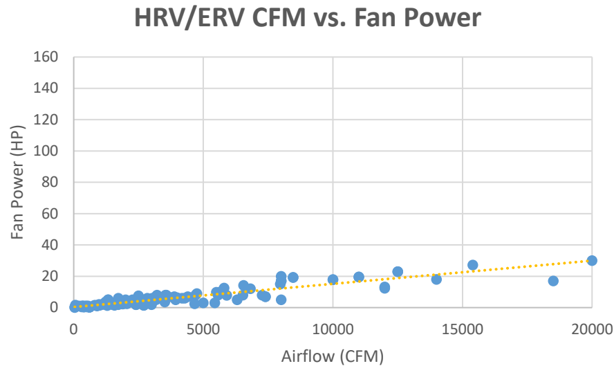
Figure 6: Airflow vs. fan power (horsepower) of air-to-air heat and energy recovery ventilators.
