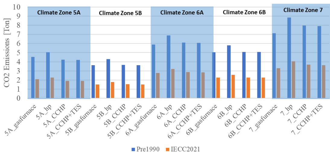
Figure 8. Heating season carbon emissions are lowest for CCHP+TES, except in the coldest climate zones.
