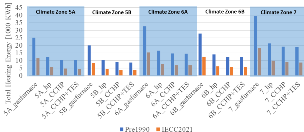
Figure 3. Annual heating energy use is reduced by CCHP and TES.
