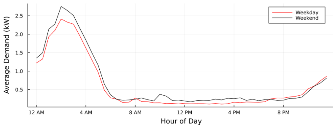
Figure 3. Average weekend and weekday loadshapes for home charging from enrolled vehicles, across February 2022.
