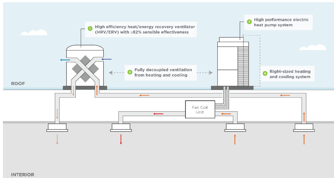
Figure 1. Very high efficiency DOAS diagram with key elements (NEEA 2022).
