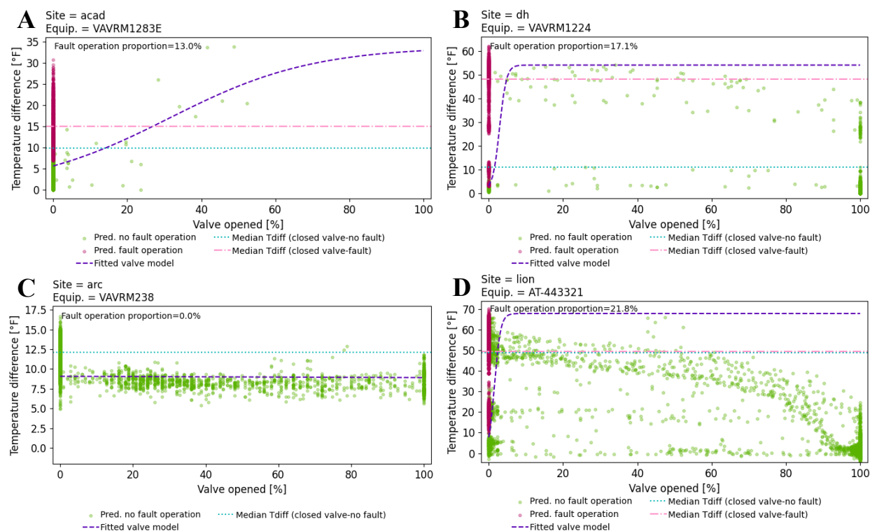
Figure 3: Operational data examples from VAV units with various faults. A), B) Passing valve fault, C) sensor fault, and D) reversed valve fault. A high median temperature difference when the valve is closed (red dots) is an indication for a potential passing valve.
