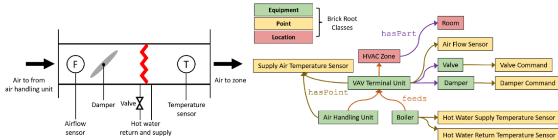
Figure 1: Left) schematic of a variable air volume (VAV) with reheat terminal unit and right) a Brick data model of the VAV terminal unit.
