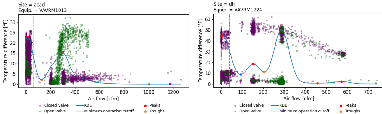
Figure 2: Temperature difference between the upstream and downstream air temperature of VAV reheat coil versus its air flow rate when reheat valve is open (green) and closed (purple). The solid blue line is the kernel density estimation (KDE) with peaks (red) and troughs (orange) highlighted. The dashed gray line indicates the calculated minimum air flow rate to consider the VAV in operating mode.
