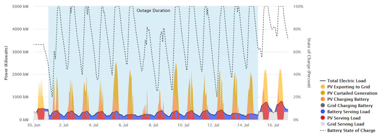
Figure 9. Summer resiliency power use and dispatch (NREL, REopt Lite Results from Golden, CO, PV and Battery Storage Financial Evaluation, Summer n.d.)
