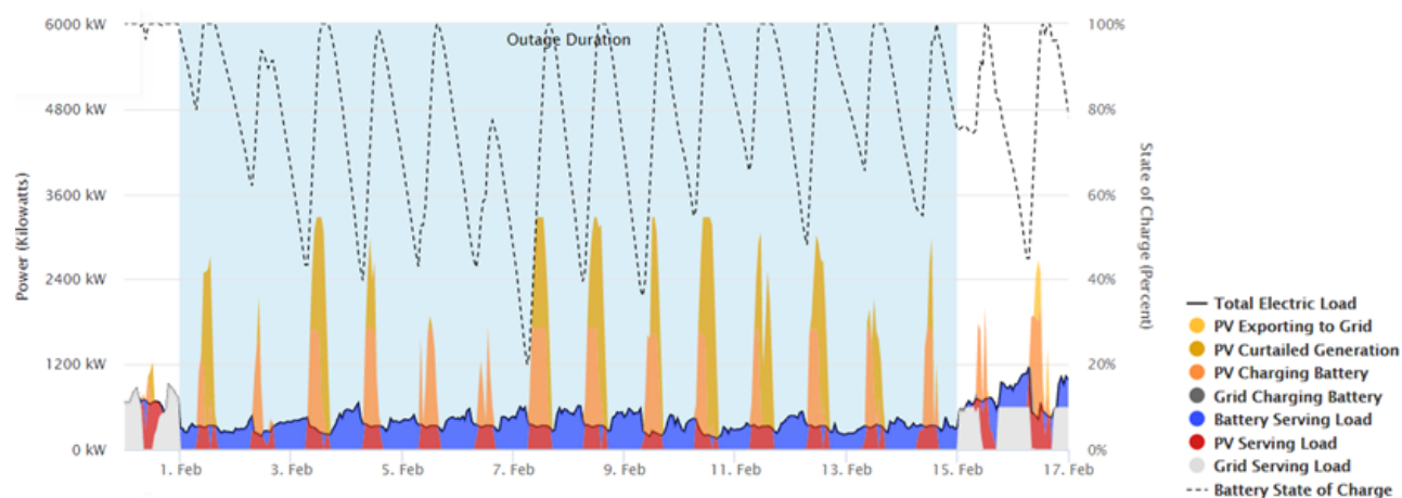
Figure 10. Winter resiliency power use and dispatch (NREL, REopt Lite Results from Golden, CO, PV and Battery Storage Financial Evaluation, Winter n.d.)
