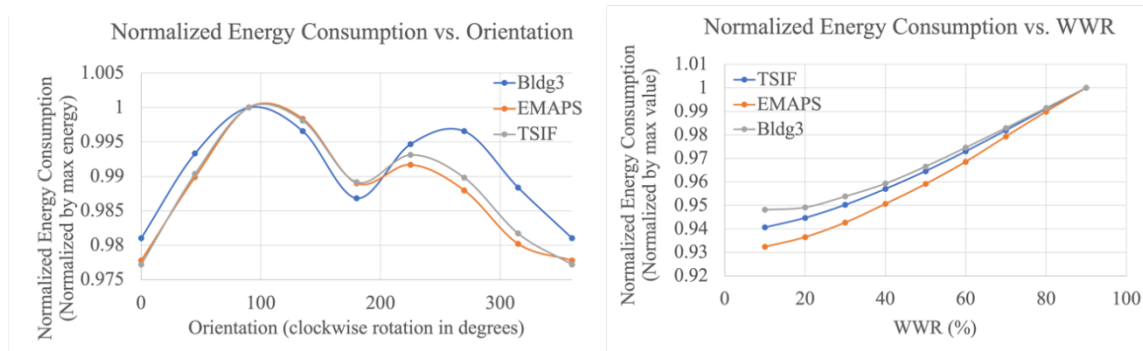
Figure 5. Normalized annual energy consumption of each building model as a function of building orientation [left] and window-to-wall ratio (WWR) [right]
