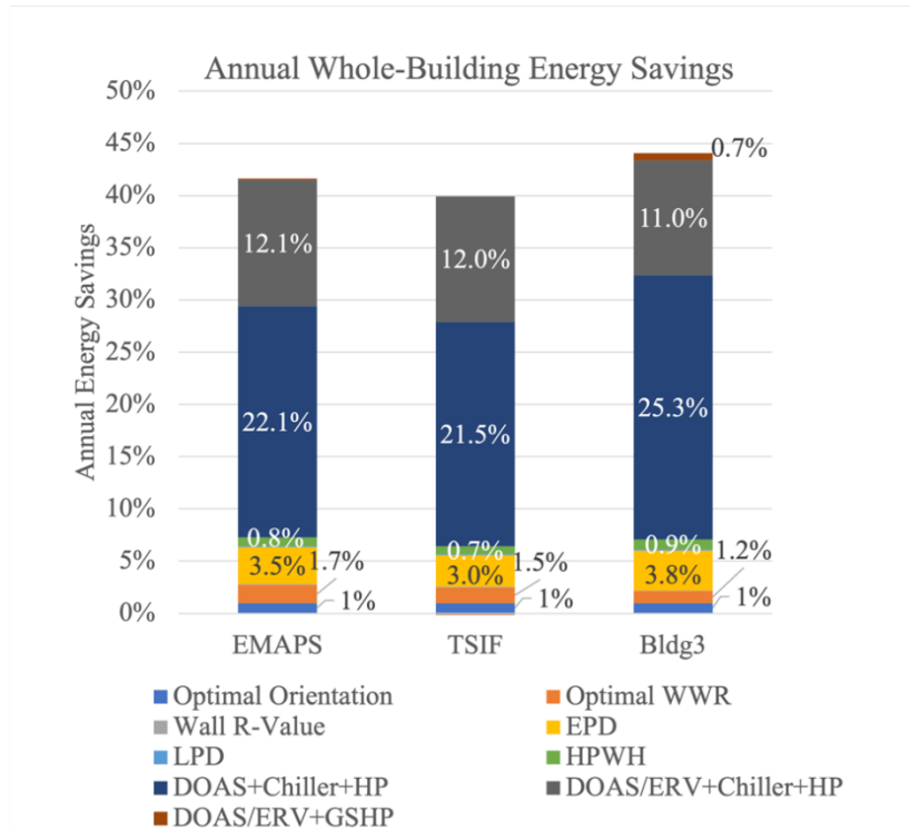
Figure 6. Annual whole-building energy savings as a function of incremental energy efficiency measures and HVAC options
