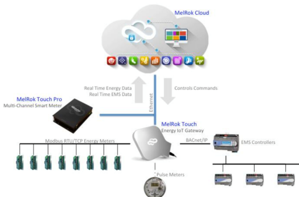
Figure 1. Overview of the Melrok technology stack that was developed and deployed at the university campus.
