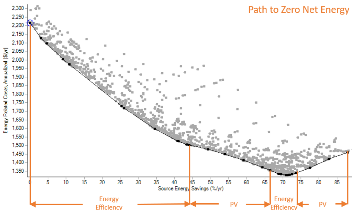
Figure 2. Example BEopt optimization output, circa 2016, for a single-family detached new construction home in Chicago.
