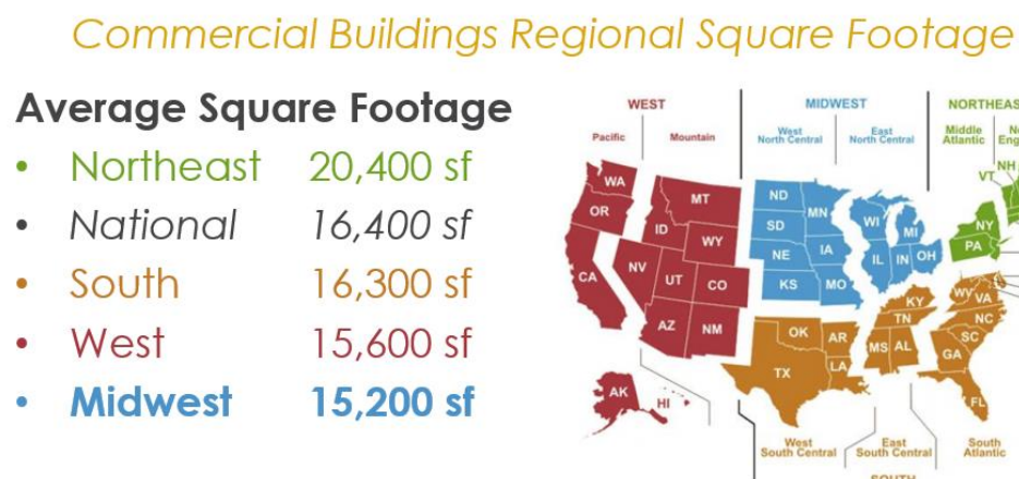
Figure 2. Average size of existing commercial buildings by region in the United States. CBECS does not include Kentucky in the Midwest. Data Source: CBECS 2018.
