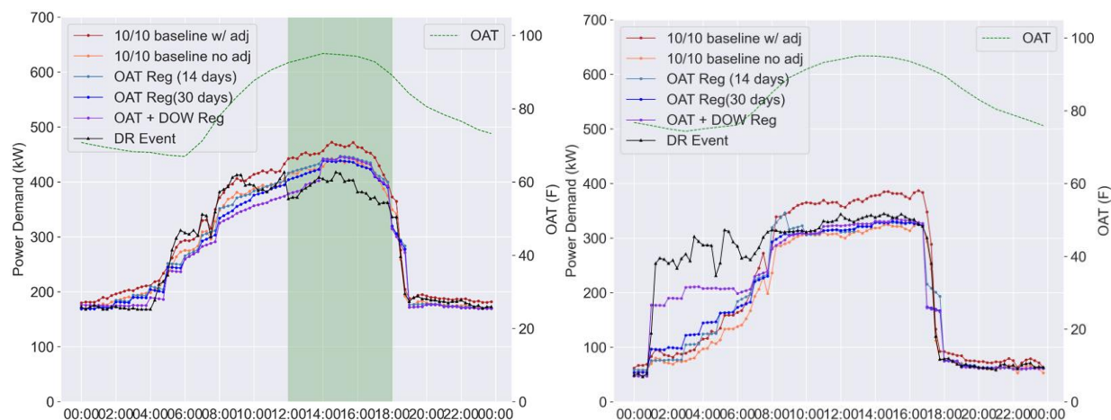
Figure 7: Representative Time-Series Plots of Actual Power and Different Counterfactual Baseline Load Shapes on a DR Event Day (Left: 7-a) and a Non-Event Day (Right: 7-b) for a Group of Medium Office Buildings
