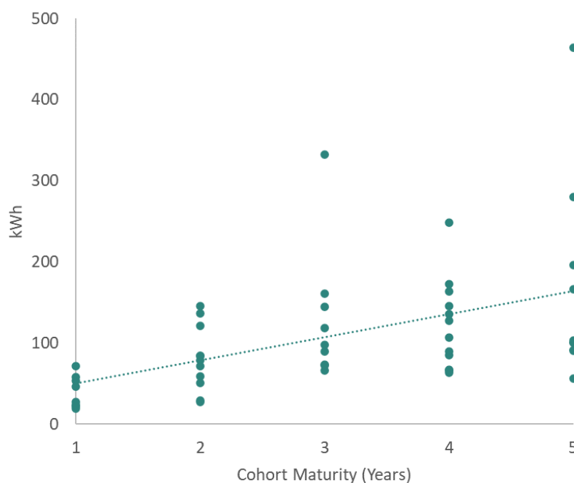
Figure 8. Unadjusted Annual Household Electric Savings by Cohort Maturity. (n=50 cohorts; Pearson's r=.48 )
