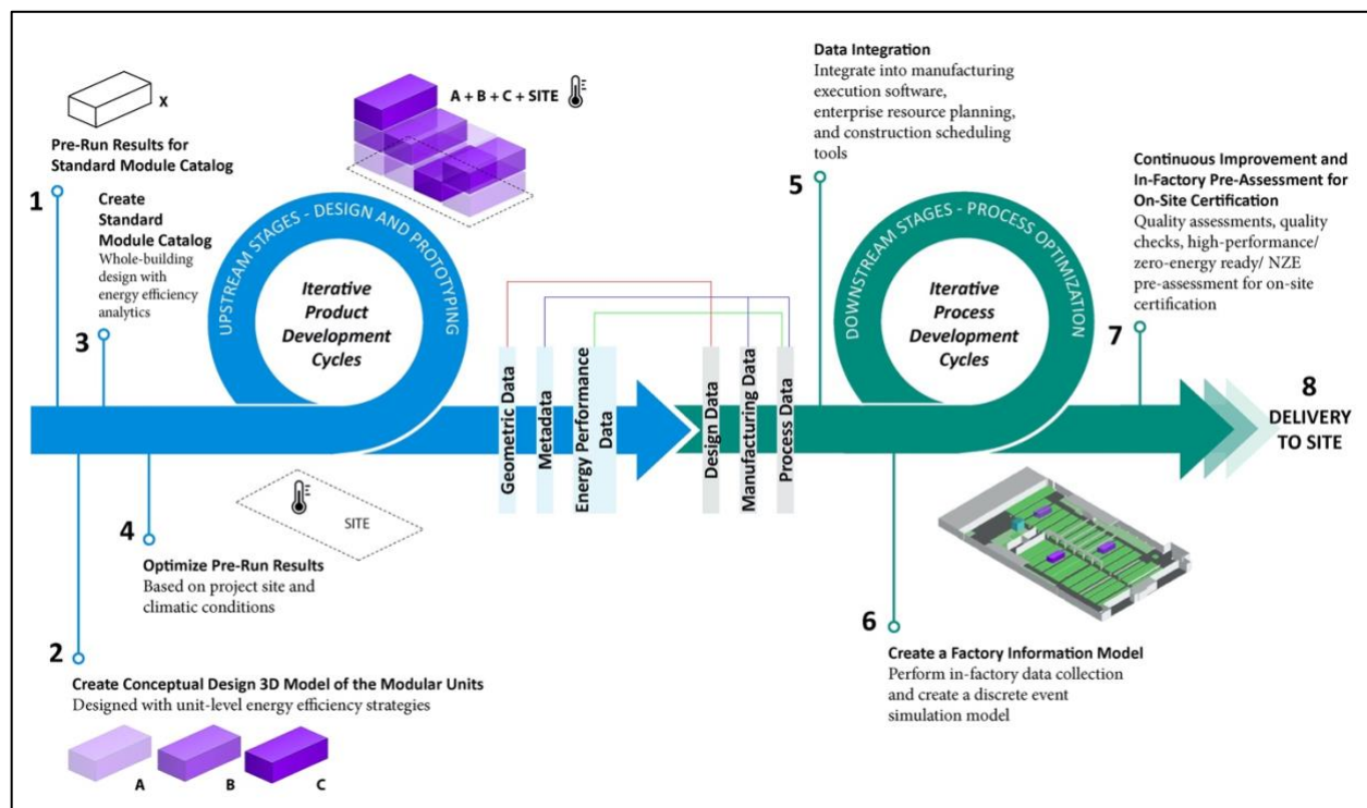
Figure 1. Integrated design-production process centered around the EMOD method, involving iterative development cycles in both upstream and downstream stages. Source: NREL.
