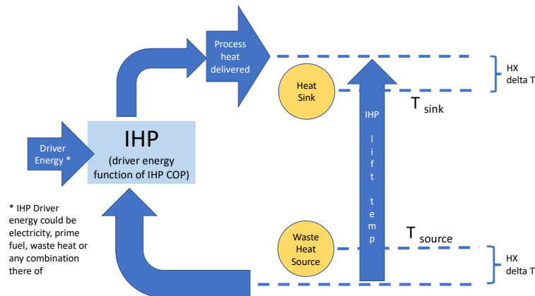
Figure 6 – Generic IHP diagram illustrating IHP lift temperature, T_{\text{source}} and T_{\text{sink}}
