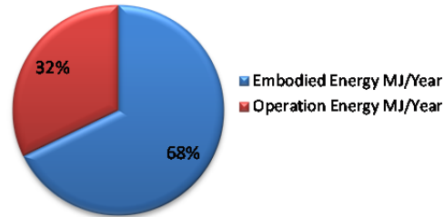
Embodied & Operational Energy Comparison
