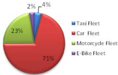
Figure 9. Structure of Private Transportation Operational Energy
