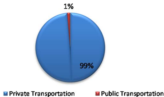
Figure8. Structure of Transportation Operational Energy Use
