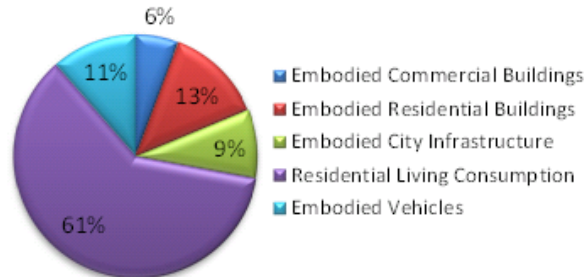
Figure7. Structure of Embodied Energy
