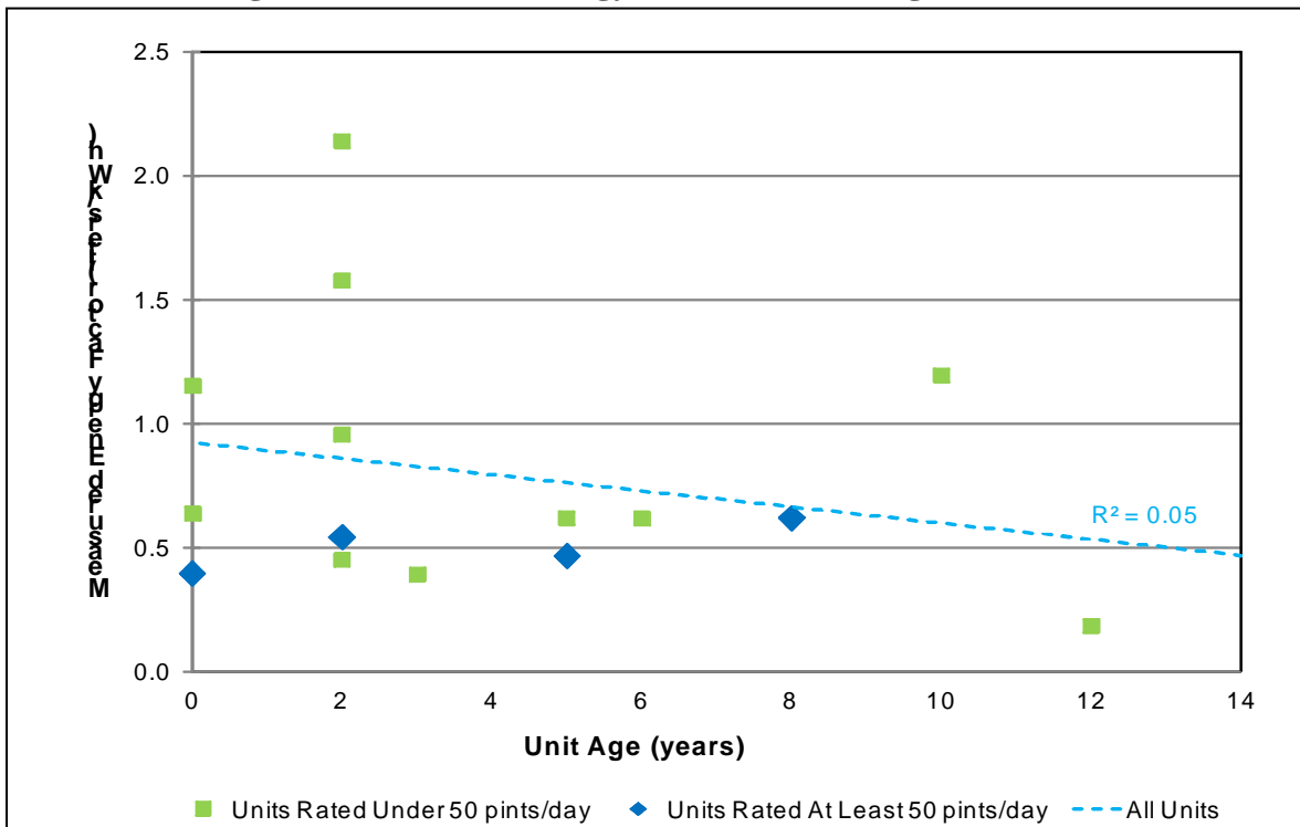
Figure 6. Measured Energy Factor Vs. Unit Age
