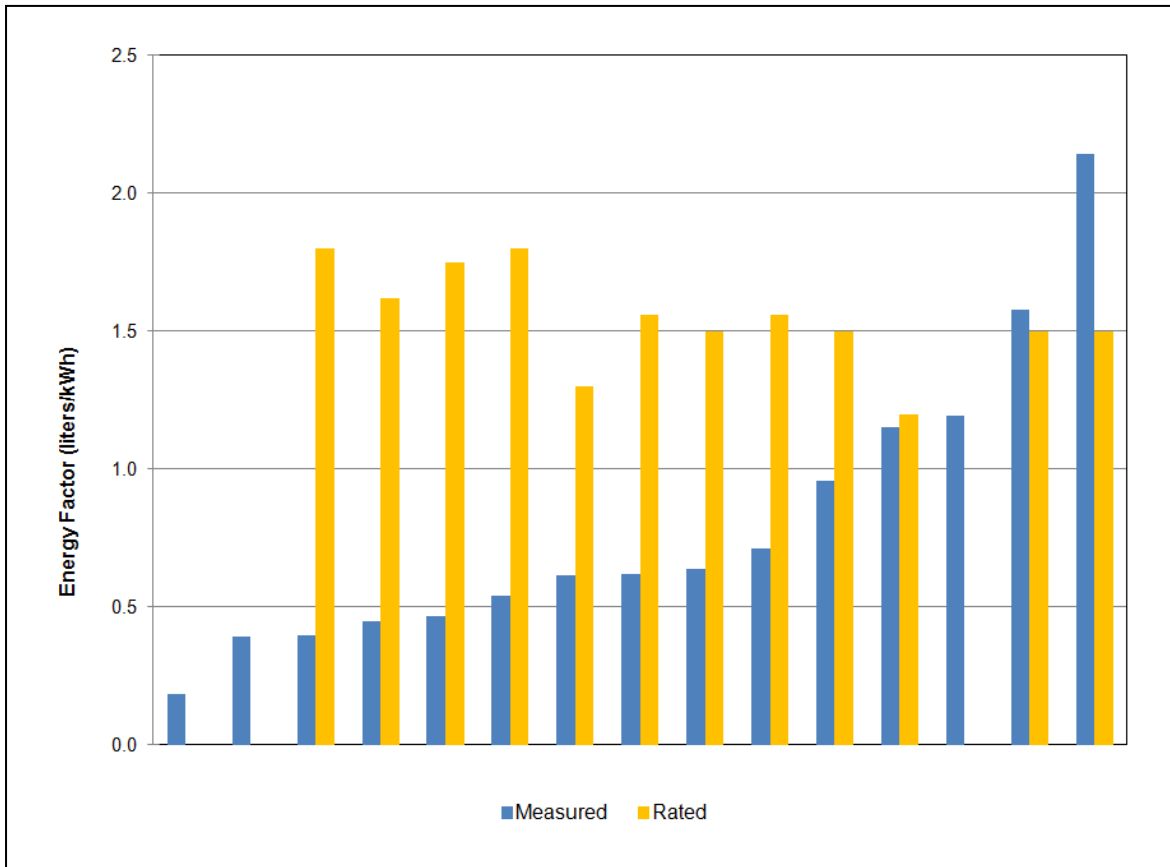
Figure 5. Comparison of Measured and Rated Energy Factors
