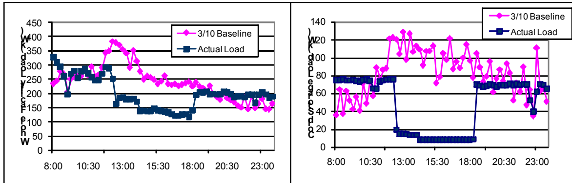
Figure 4: Demand Reduction in Refrigerated Warehouse
