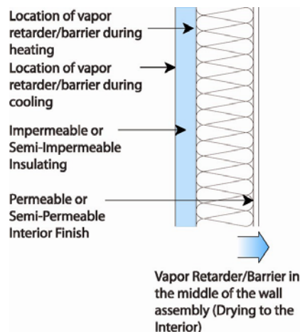
Figure 3. Vapor Control Layer in the Center of the Assembly
