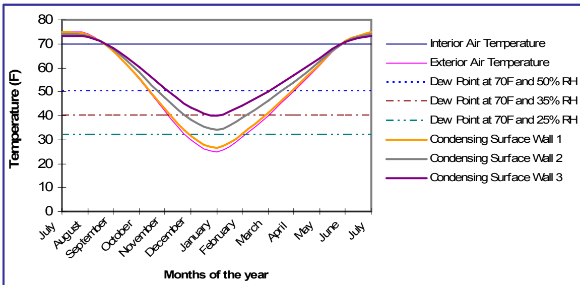
Figure 5. Condensing Surface Temperature Compared to Dew Point
