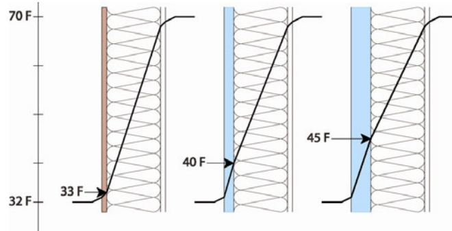
Figure 4. Thermal Gradient across Wall Assemblies
