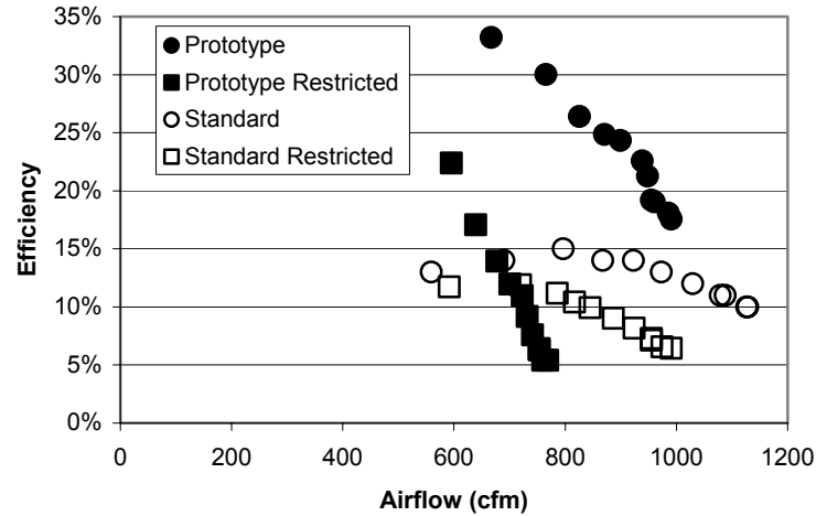
Figure 8. Reduction in Air Flow and Efficiency Due to Inlet Restriction
