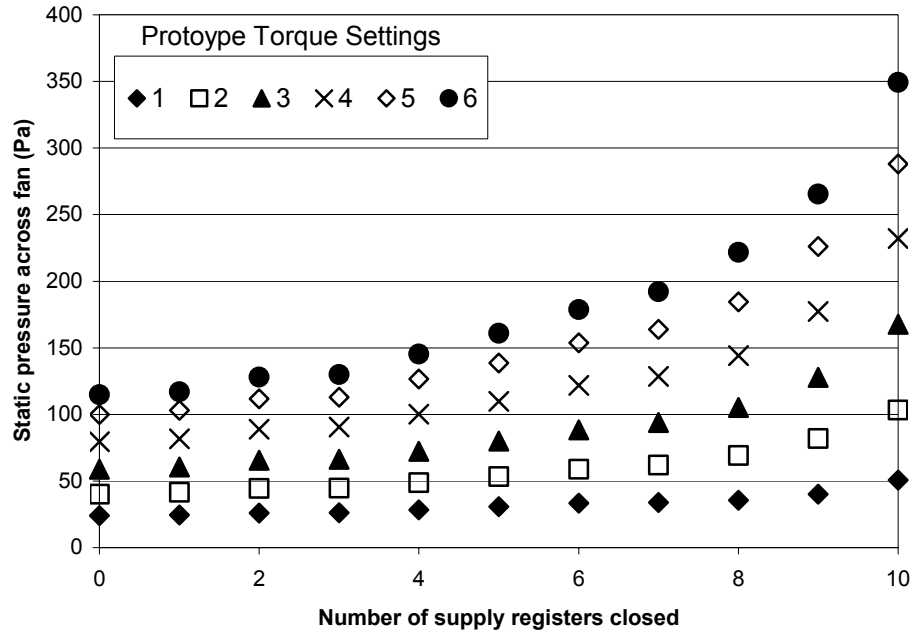
Figure 4. Static Pressure Changes Due to System Flow Resistance (Number of Closed Registers)
