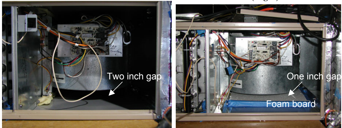
Figure 2. Standard Fan in Cabinet with No Restriction (Left) And With Added Foam Board Restriction (Right)
