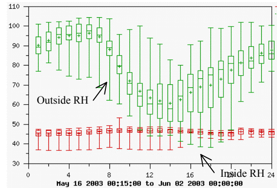
Case 4 OA plus 10/20 controller plus dehumidifier
