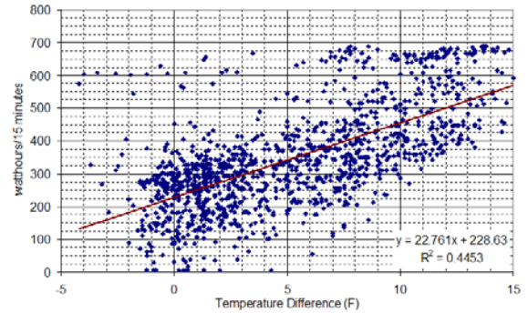
Case 6a ERV1 (Balanced)
