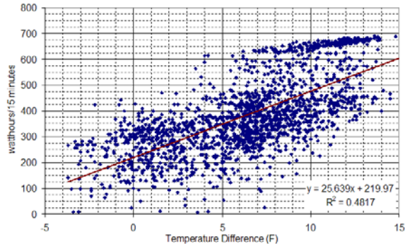
Case 6b ERV2 – Different media (Balanced)
