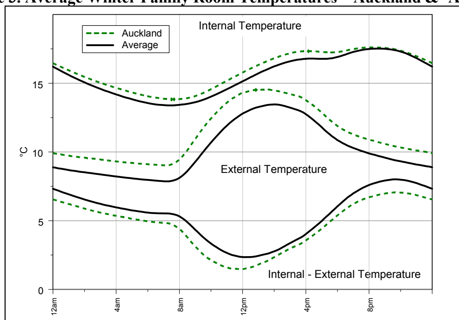
Figure 3. Average Winter Family Room Temperatures – Auckland & ‘Average’
