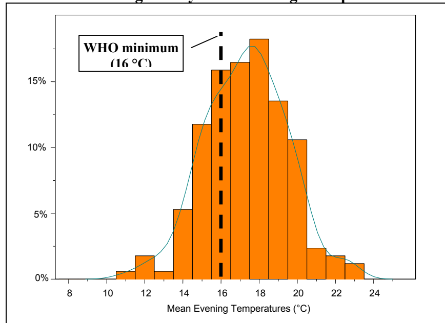
Figure 4. Winter Evening Family Room Average Temperature Distribution
