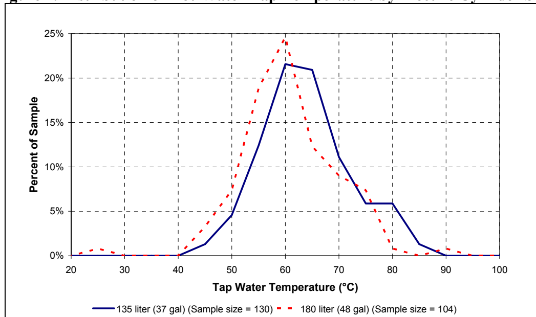
Figure 2. Distribution of Hot-Water Tap Temperature by Electric Cylinder Size
