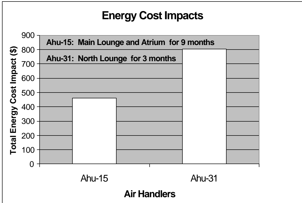
Figure 1 Sample of estimated cost impacts for two air handlers in a large hotel. The outside air dampers for both air handling units were not opening fully, resulting in loss of economizing when available and incurring a cooling-energy penalty
