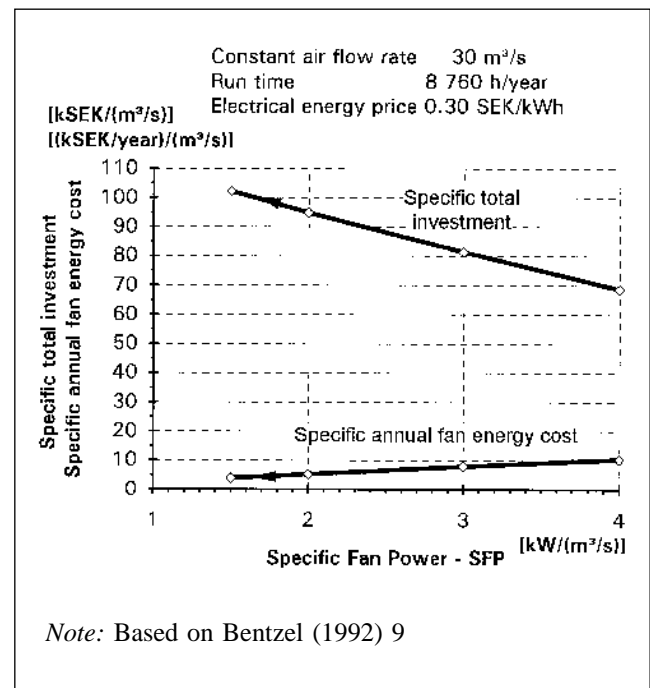
Figure 2. Specific Total Investment and Specific Annual Fan Energy Cost for the Air Distribution System Solutions Studied in the Pre-study. 1 SEK ≈ USD 0.17
