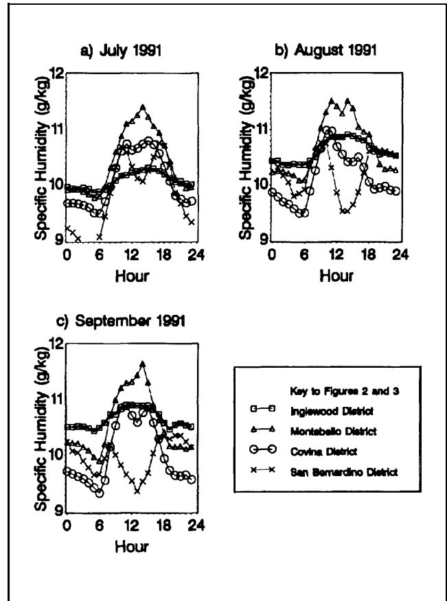
Figure 3. Monthly Average Diurnal Variations of Specific Humidity at Four SCE Weather Stations for (a) July, (b) August, and (c) September, 1991
