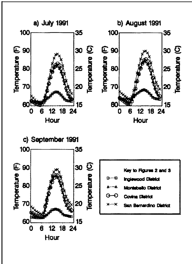
Figure 2. Monthly Average Diurnal Variations of Ambient Drybulb Temperature at Four SCE Weather Stations for (a) July, (b) August, and (c) September, 1991
