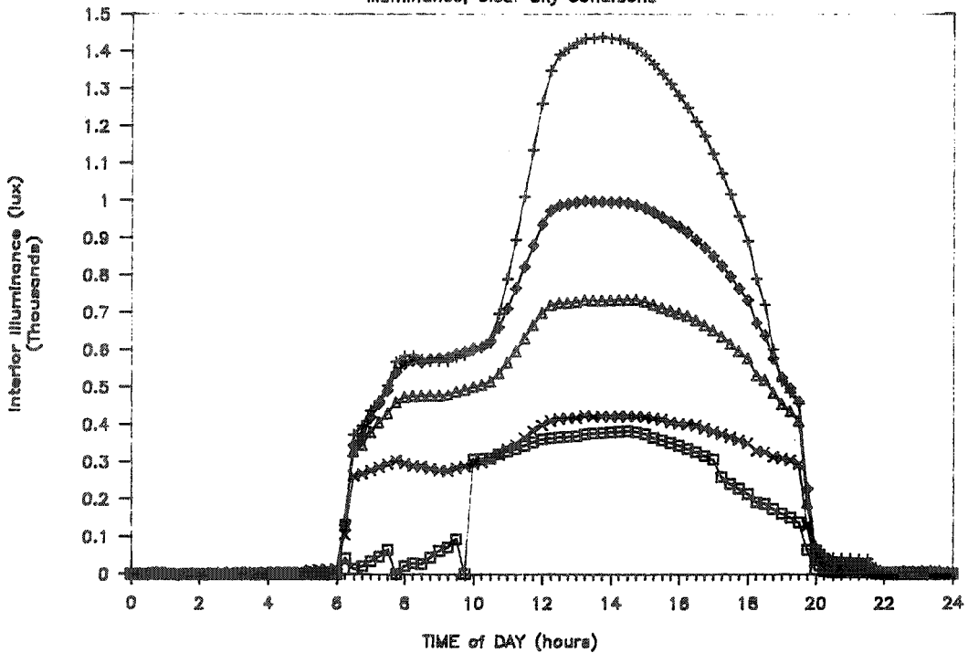
Figure 2. Interior Illuminance Values for a Typical Clear Summer Days: a) South Exterior Zone; b) North Exterior Zone.
