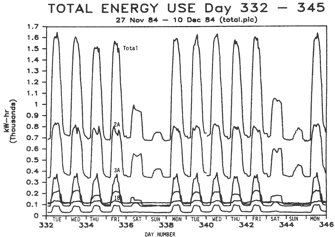
Figure 4. Hourly electrical energy use for the total building and main meters (1A, 1B, 2A, 3A, & 4A) for the period 27 November through 10 December 1984.
