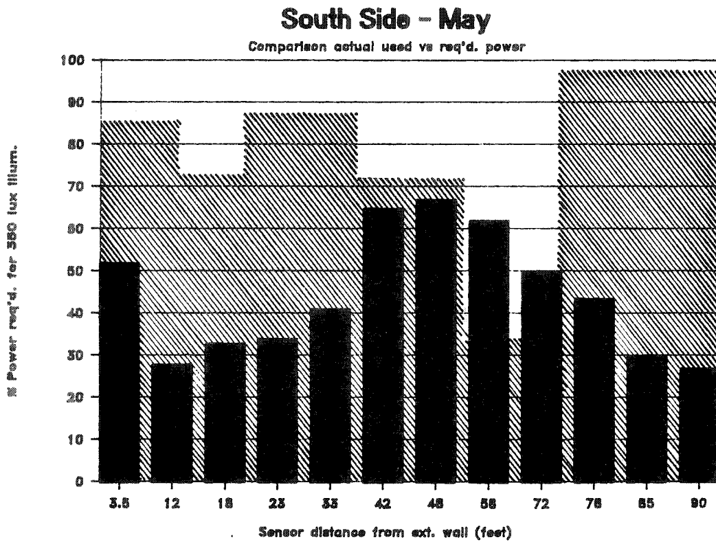
Figure 3. Potential dimming for daytime occupied hours. vs. observed dimming for the third floor south and north sides shown as a fraction of the full electrical lighting power
