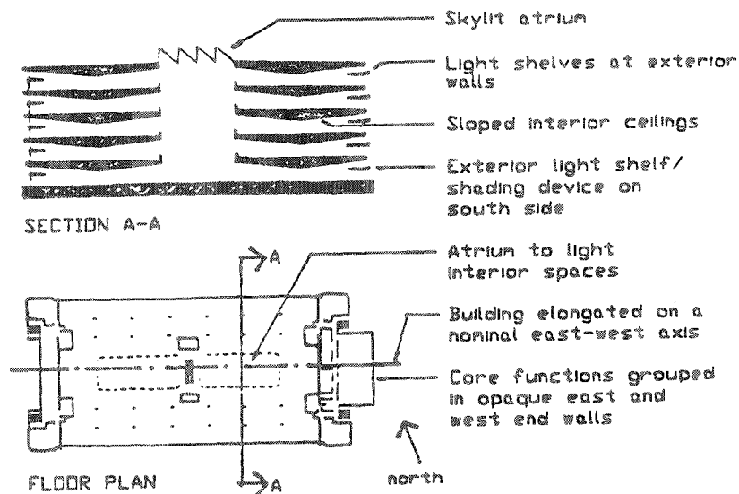
Figure 1. Section and Plan of the Building.
