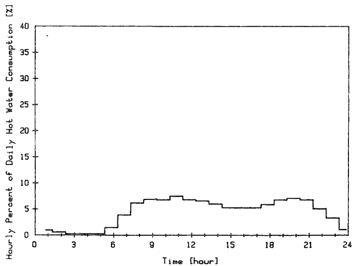
Figure 2. Comparison of domestic hot water profiles: a) RAND 1974, based on 21 New Jersey apartments, b) NSDN 1981, based on 15 single-family houses and 202 apartments (in three apartment buildings) over six-month period, and c) Holly Court 1985, based on 48 apartments (in four apartment buildings) over a six-month period. [Source for RAND and NSDN profiles: Barvir et al., 1981].
