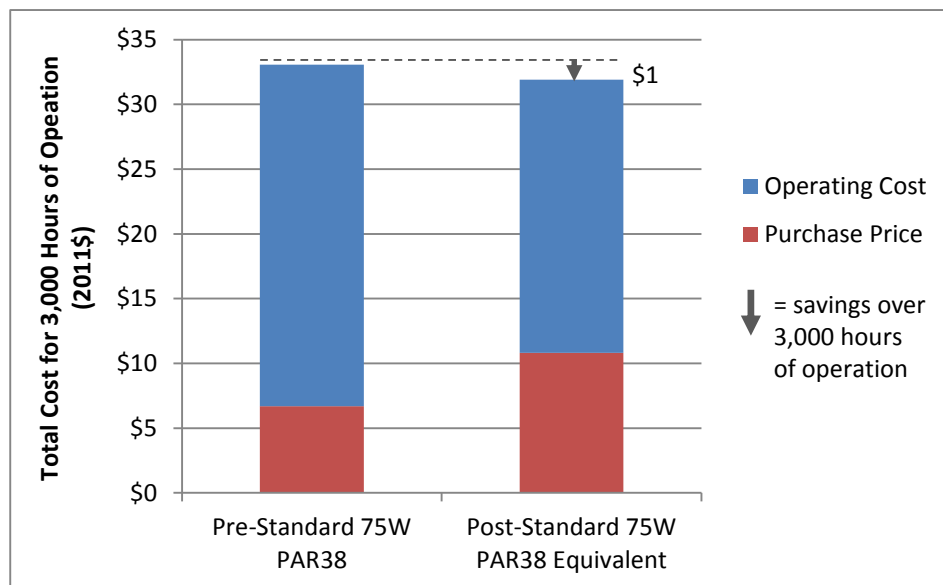
Figure 35. Comparison of Total Cost of Pre-Standard and Post-Standard 75W Equivalent PAR38 Lamps for 3,000 Hours of Operation
